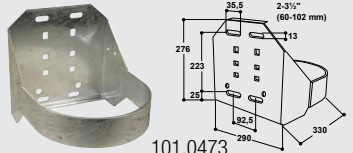
101.0473
