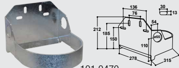
101.0470
