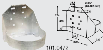
101.0472
